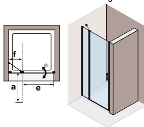
45 Art. 8U-4TN2 L Anschlag links
